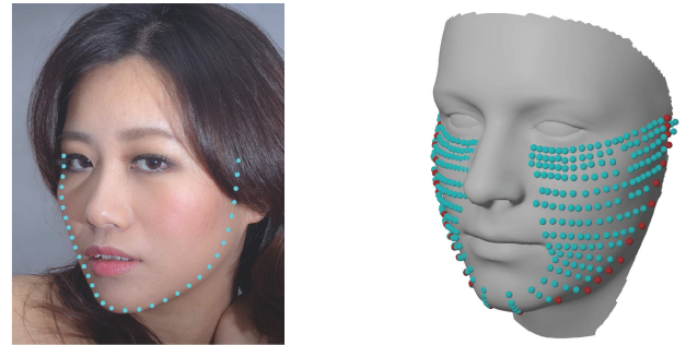
Fig. 4 For a non-frontal face image (left), we dynamically update the 3D face silhouette landmarks (red) according to the current estimated rotation, to give better correspondence with the detected 2D silhouette landmarks (left, cyan).
